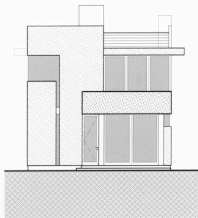
North elevation
