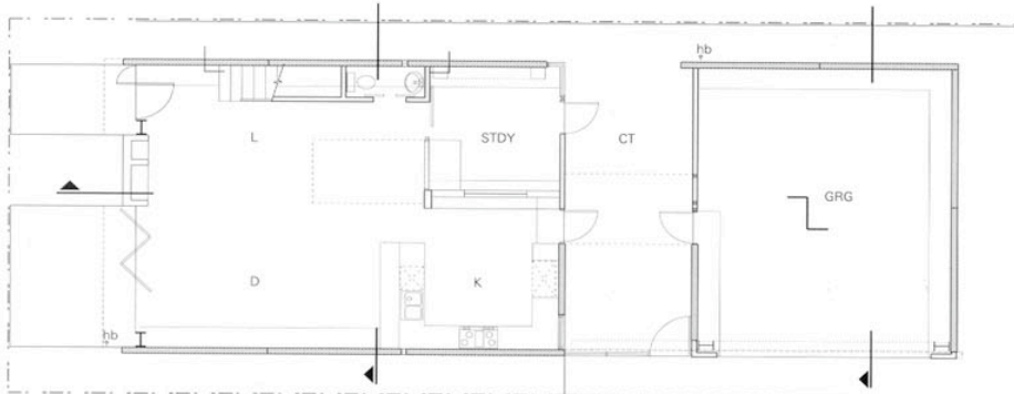
First floor
